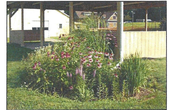
This rain garden in Vernon, CT was constructed as a demonstration project to treat and infiltrate runoff from an outdoor pavilion. Photo: USDA NRCS
